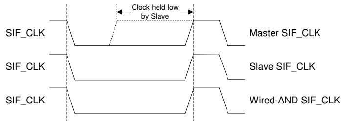
Figure 35: Clock Stretching
