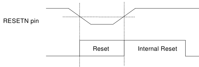
Figure 10: External Reset
