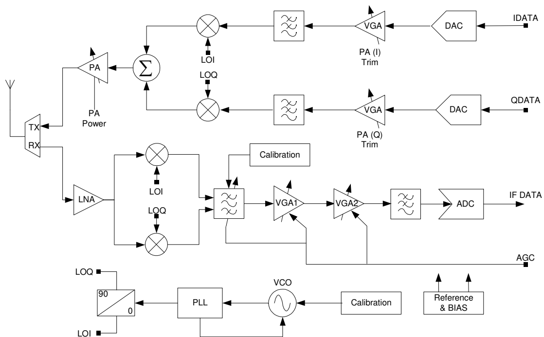
Figure 12: Radio Architecture
