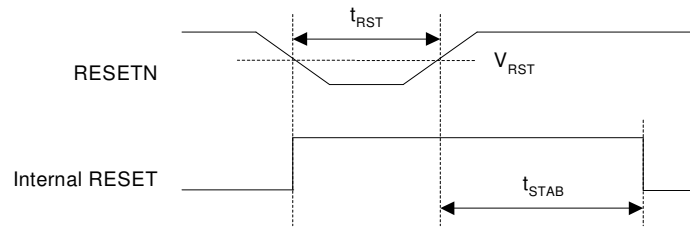
Figure 39: External Reset
