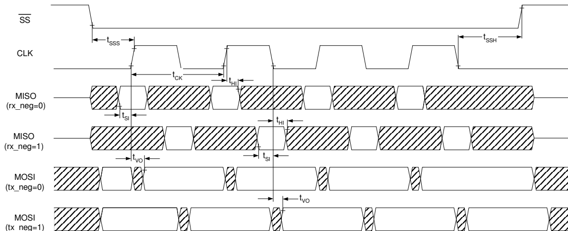
Figure 40: SPI Timing (Master)
