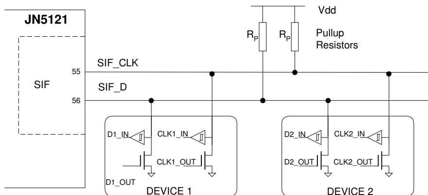
Figure 33: Connection Details
